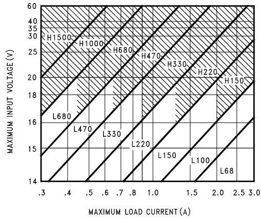
Figure 5. LM2576(HV)-12
