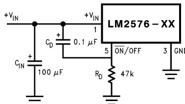
Figure 12. Delayed Startup
