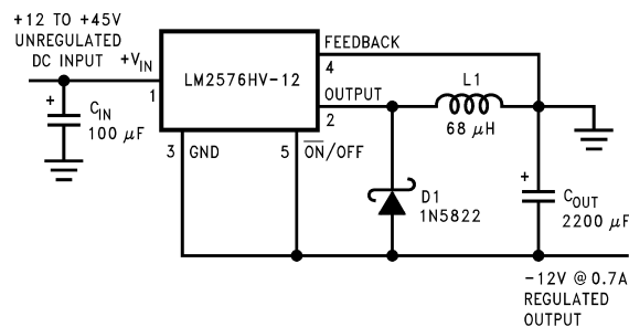
Figure 8. Inverting Buck-Boost Develops -12V
