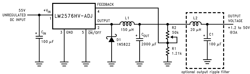
Figure 13. 1.2V to 55V Adjustable 3A Power Supply with Low Output Ripple
