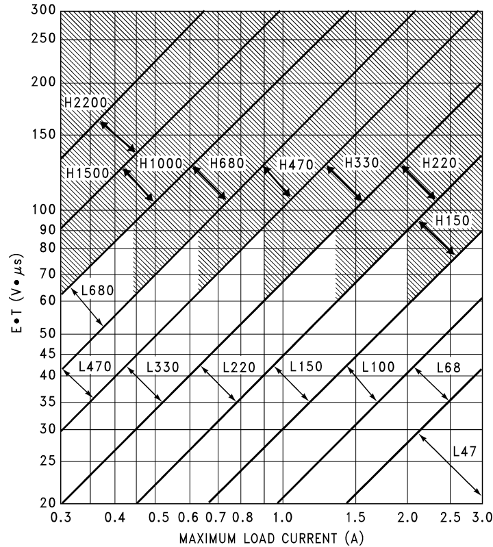
Figure 7. LM2576(HV)-ADJ
