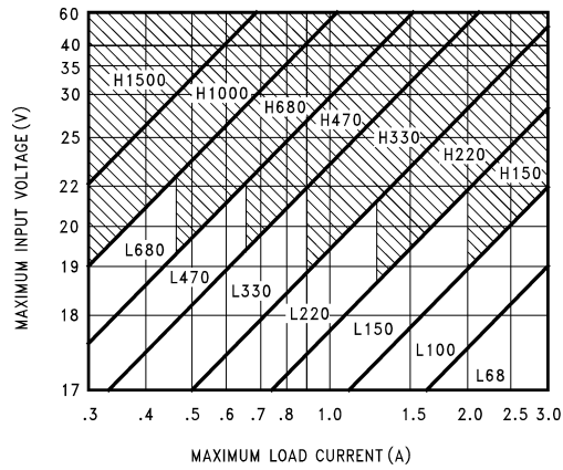
Figure 6. LM2576(HV)-15
