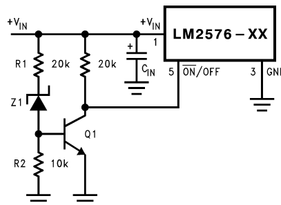
Figure 10. Undervoltage Lockout for Buck Circuit
