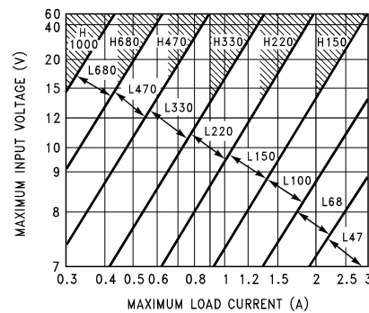
Figure 4. LM2576(HV)-5.0
