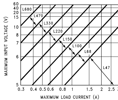
Figure 3. LM2576(HV)-3.3
