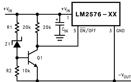
Figure 11. Undervoltage Lockout for Buck-Boost Circuit
